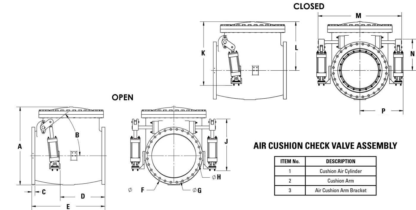
AIR CUSHION CHECK VALVE - OPEN
