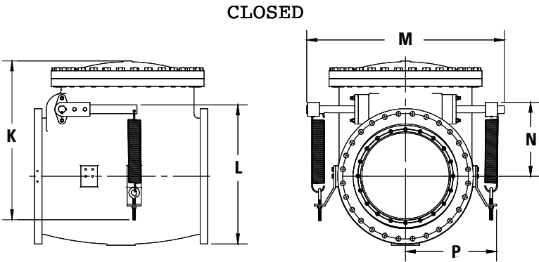
LEVER & SPRING CHECK VALVE - CLOSED
