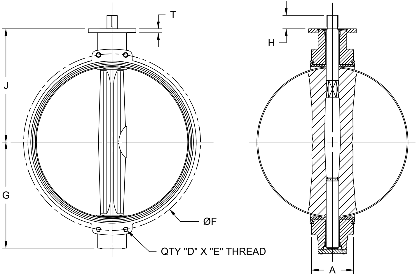
DIMENSIONS (Inches)
