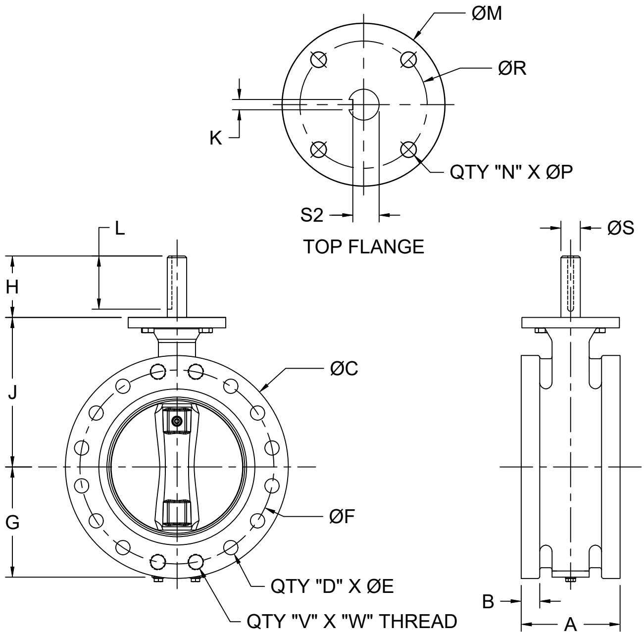
DIMENSIONS (Inches)
