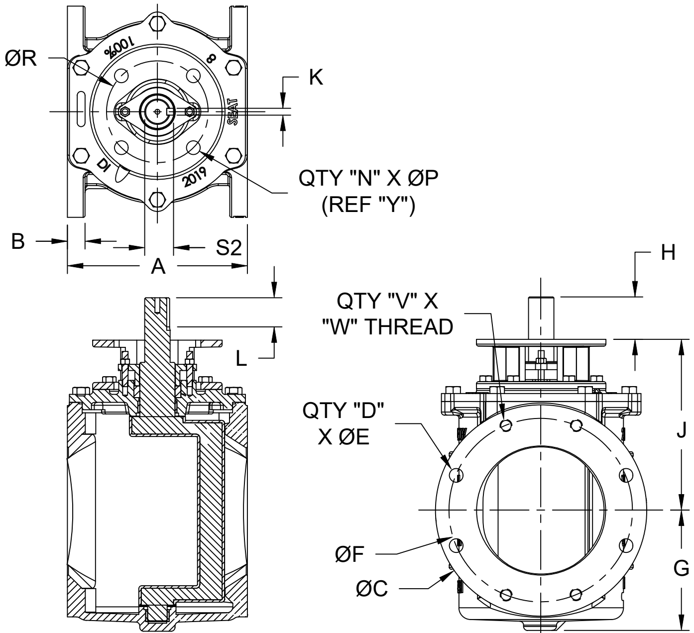
DIMENSIONS (Inches)
