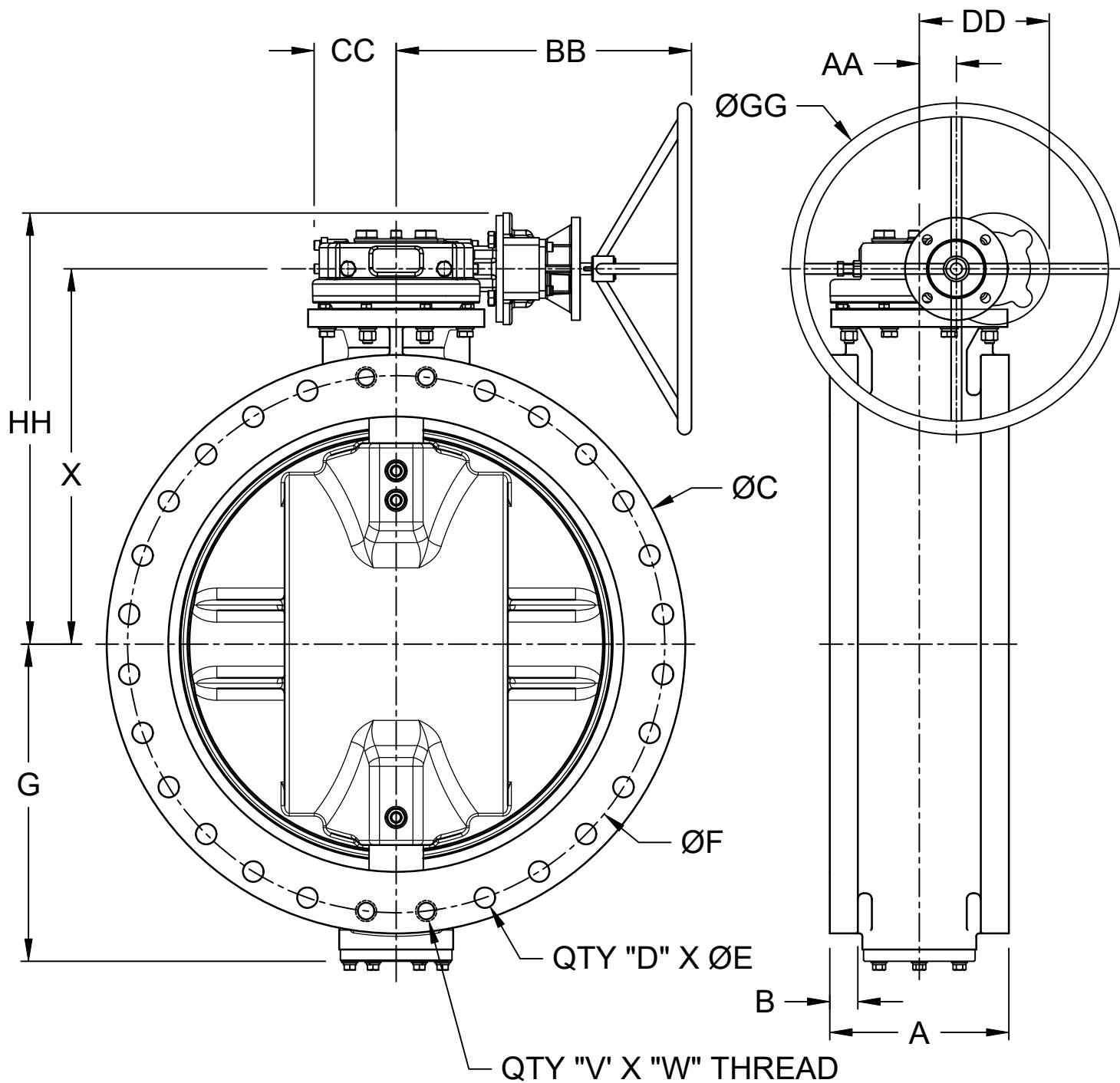
DIMENSIONS (Inches)
