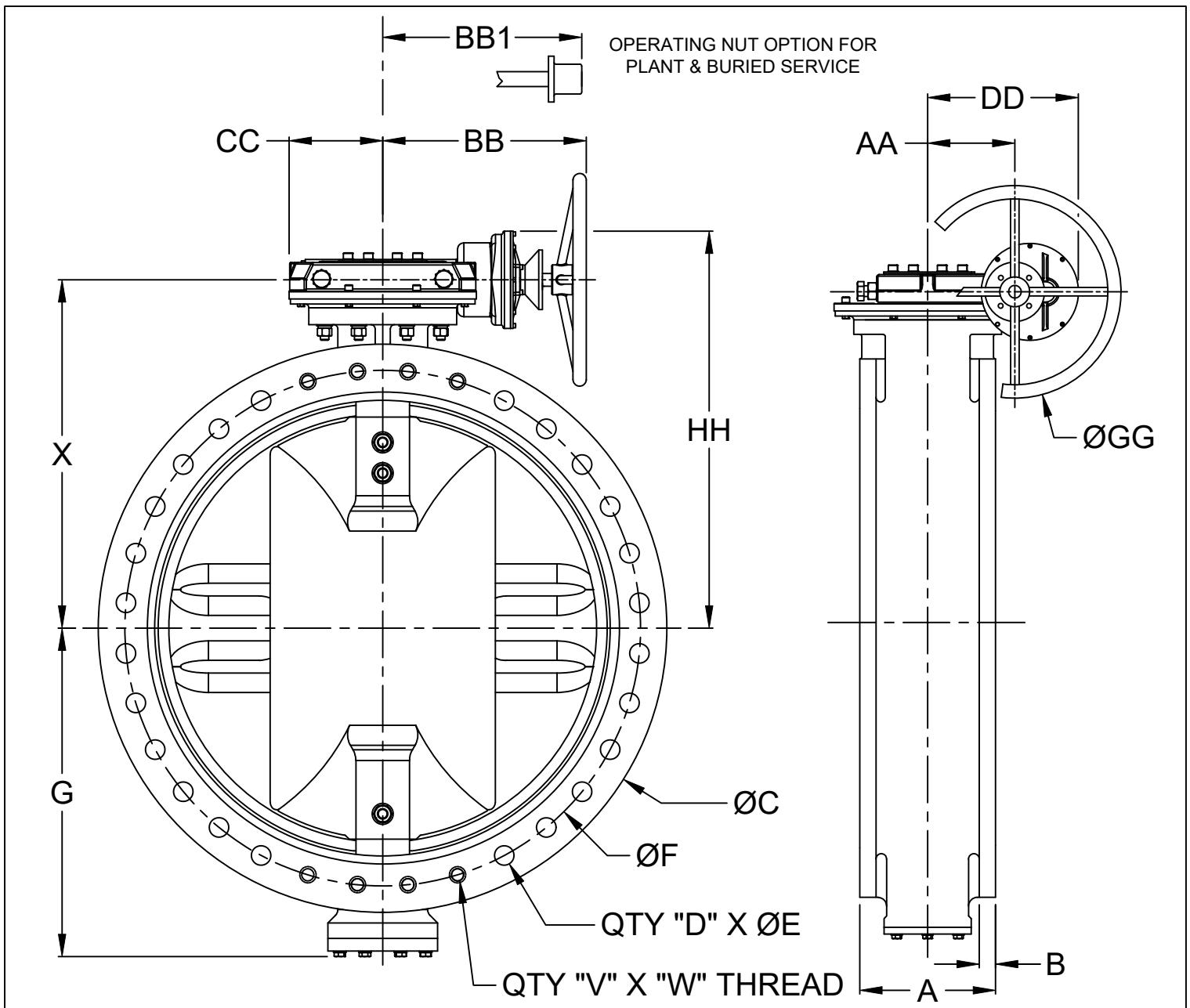
DIMENSIONS (Inches)
