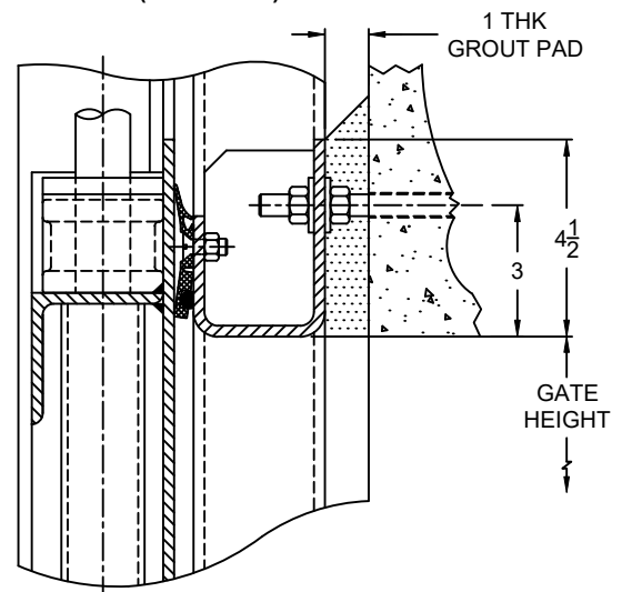
SECTION VIEW - C CROSS RAIL (OPTIONAL NON-RISING STEM)
