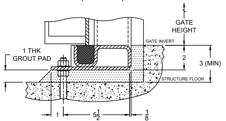
SECTION VIEW - B SURFACE MOUNTED FLUSHBOTTOM RAIL (OPTIONAL)
