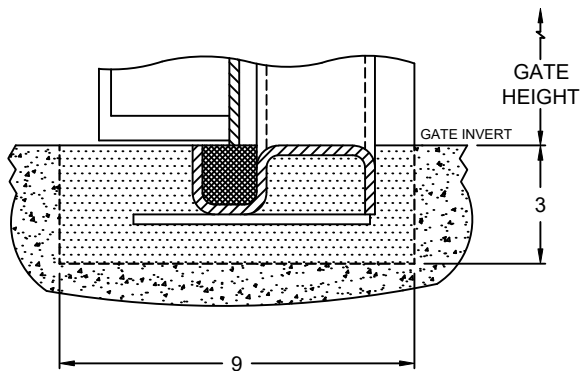
SECTION VIEW - B EMBEDDED FLUSHBOTTOM RAIL (OPTIONAL)
