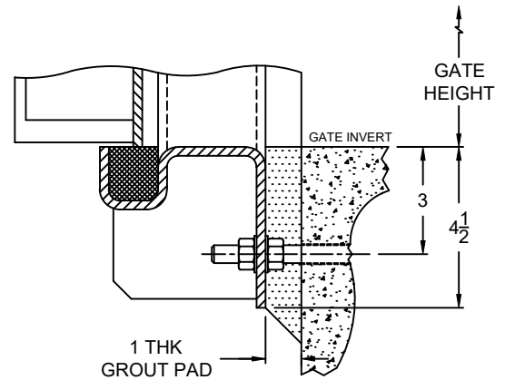
SECTION VIEW - B FACE MOUNTED FLUSHBOTTOM RAIL (STANDARD)
