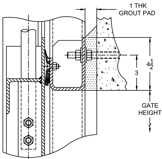
SECTION VIEW - C CROSS RAIL (STANDARD RISING STEM)
