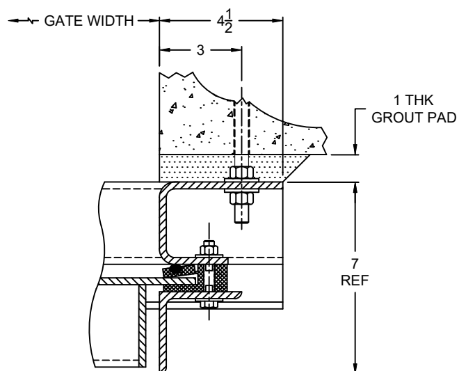
SECTION VIEW - A FACE MOUNTED GUIDE RAIL
