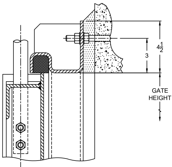
SECTION VIEW - C FLUSHTOP RAIL (RISING STEM)
