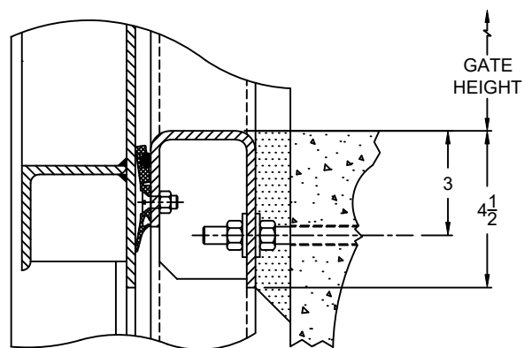
SECTION VIEW - B CROSS RAIL
