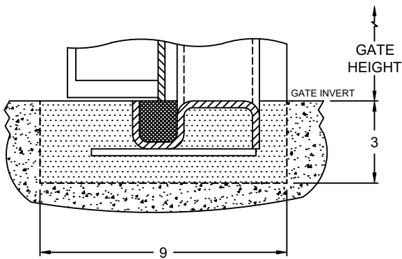
SECTION VIEW - B EMBEDDED FLUSHBOTTOM RAIL (OPTIONAL)
