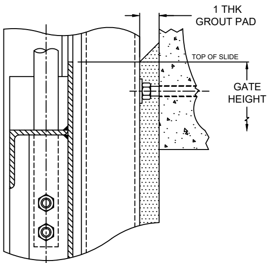
SECTION VIEW - C TOP OF SLIDE (STANDARD RISING STEM)
