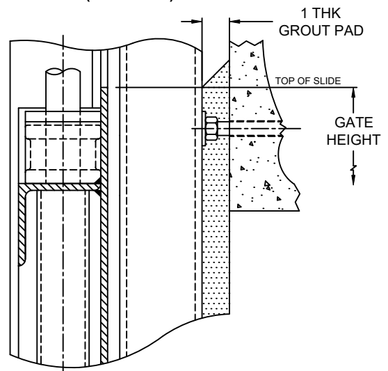
SECTION VIEW - C TOP OF SLIDE (OPTIONAL NON-RISING STEM)
