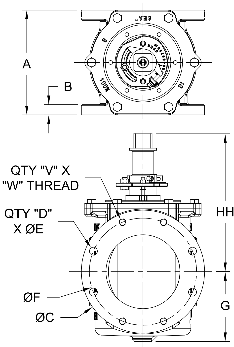
DIMENSIONS (Inches)
