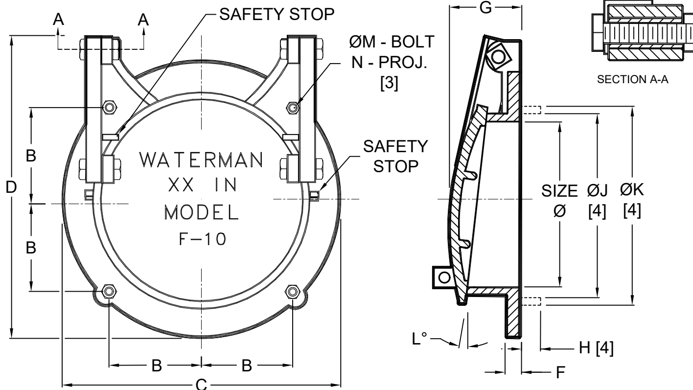
DIMENSIONS (Inches)
