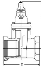
8057 Threaded Ends 2"-3"
