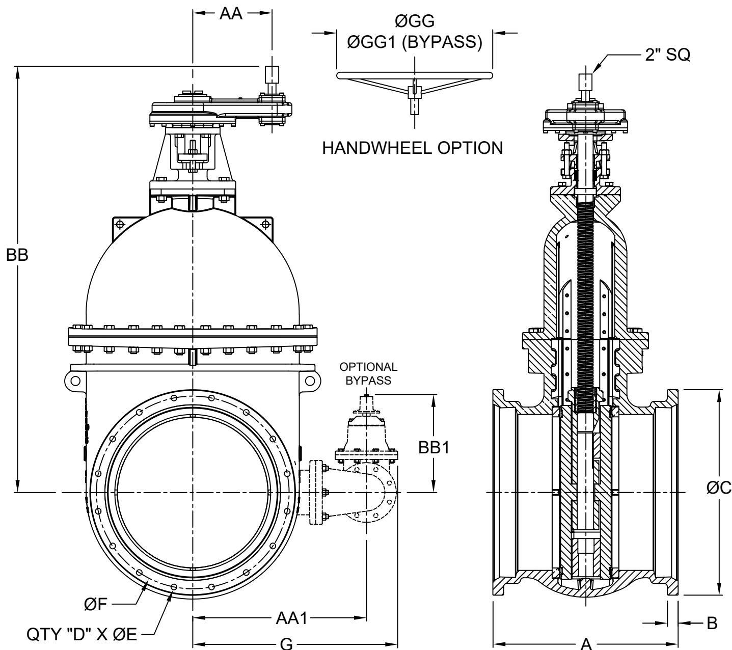
DIMENSIONS (Inches)
