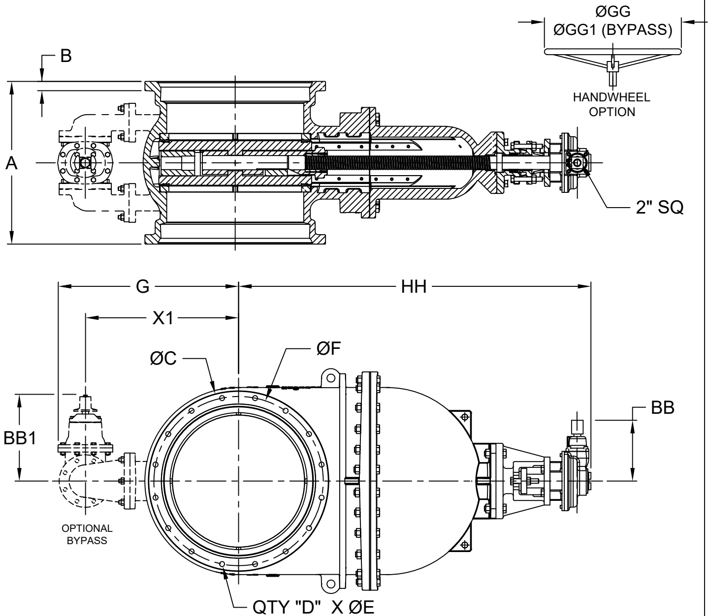
DIMENSIONS (Inches)
