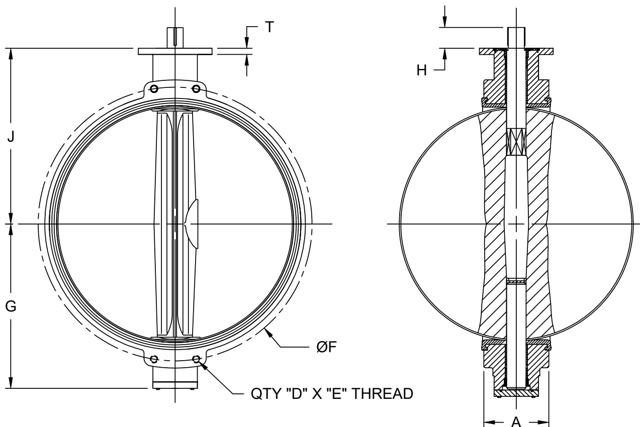
DIMENSIONS (Inches)
