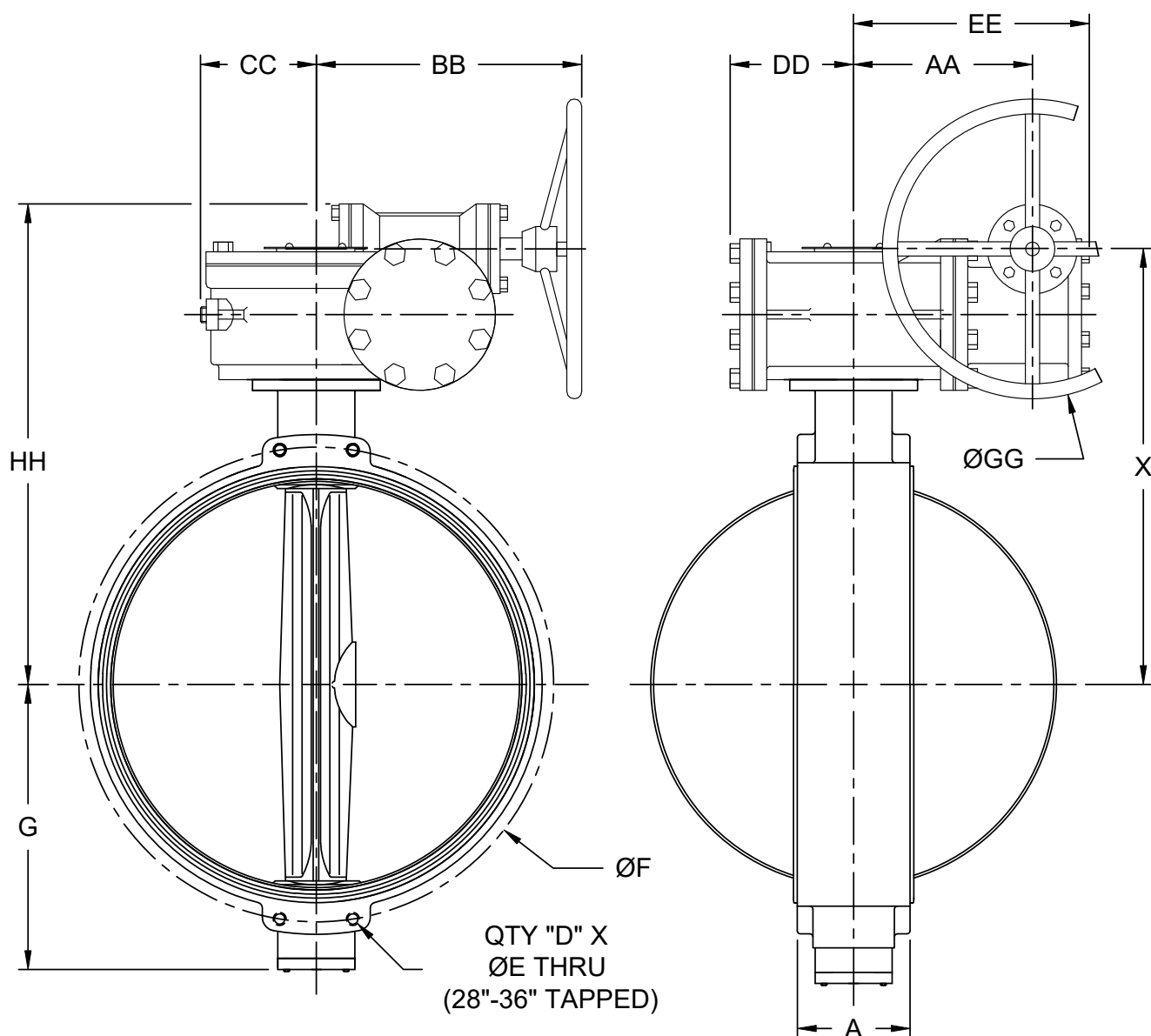
DIMENSIONS (Inches)
