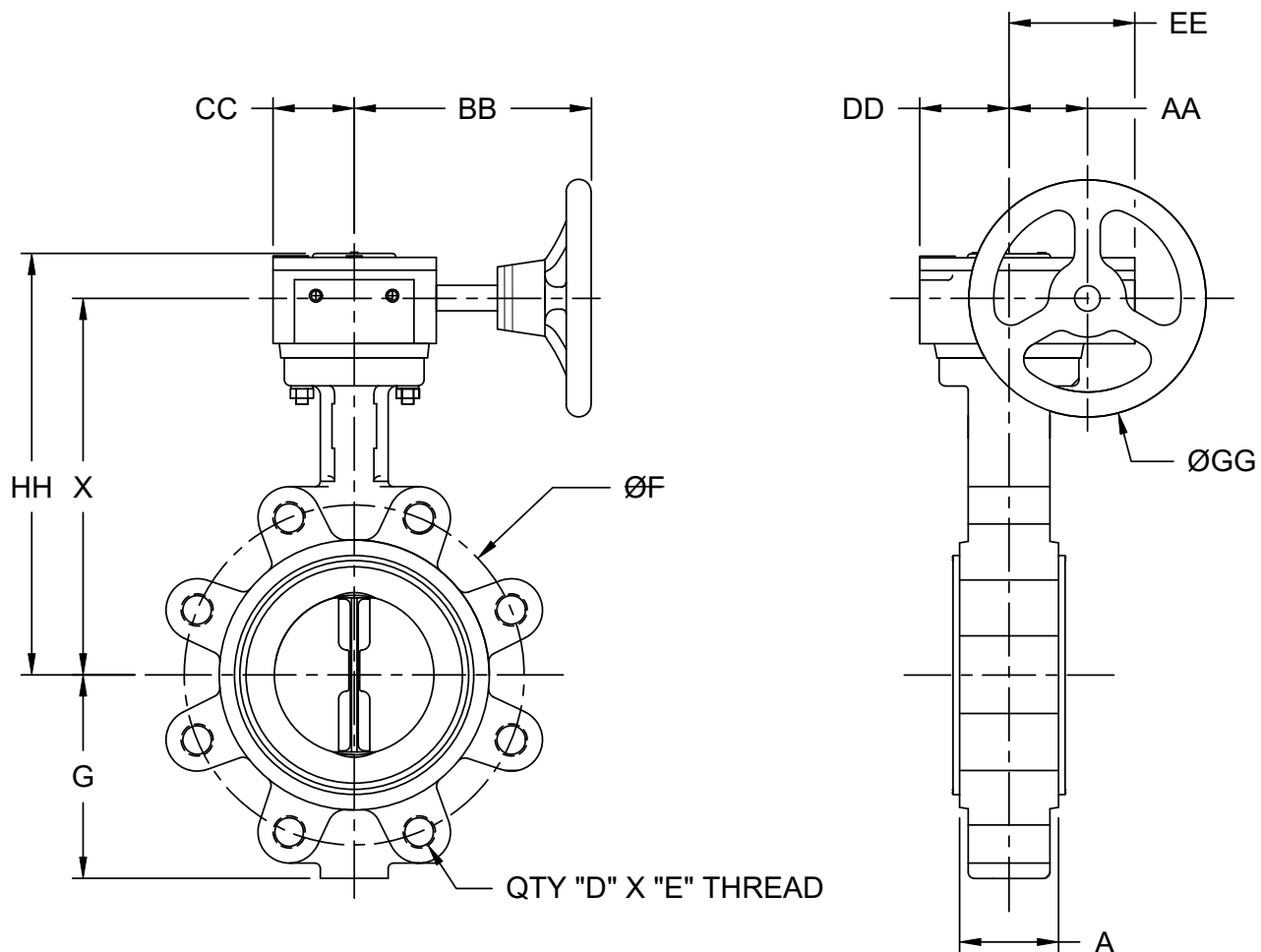
DIMENSIONS (Inches)
