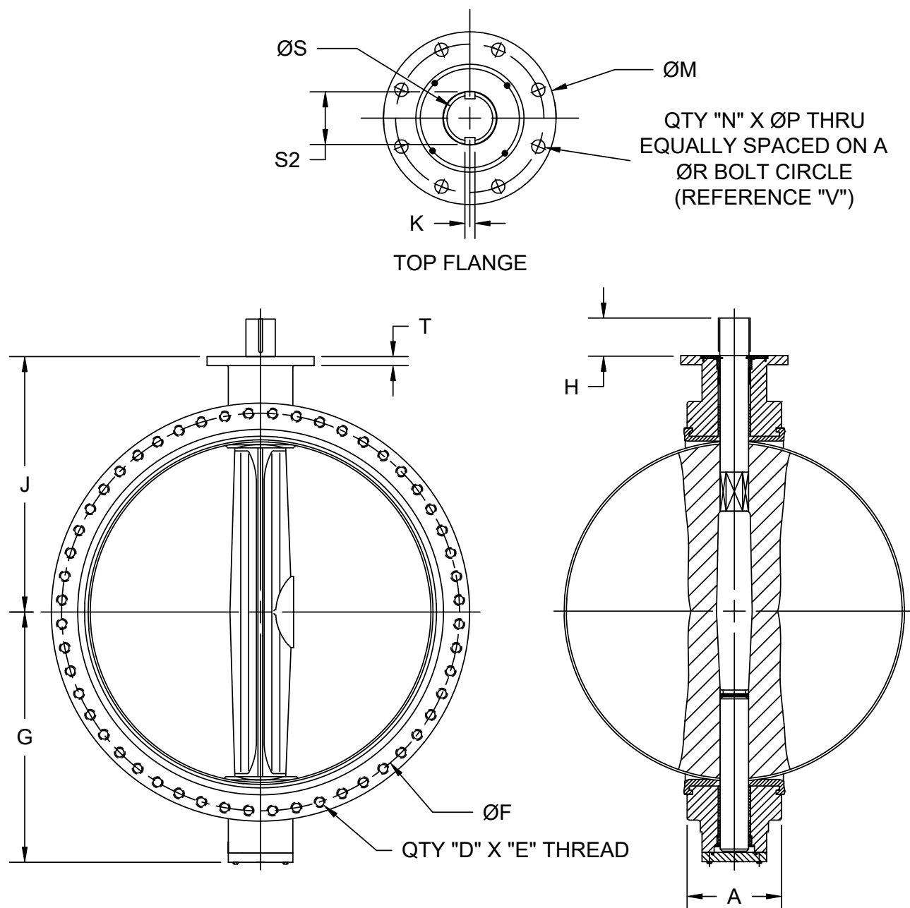
DIMENSIONS (Inches)
