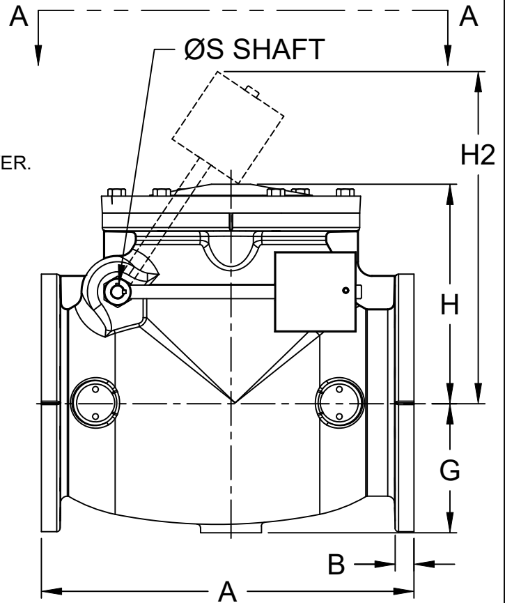
DIMENSIONS (Inches)
