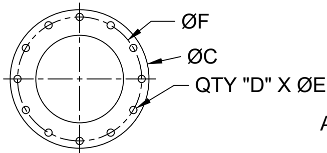
FLANGE DRILLING
