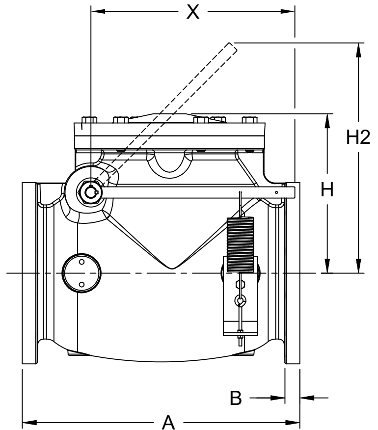
DIMENSIONS (Inches)
