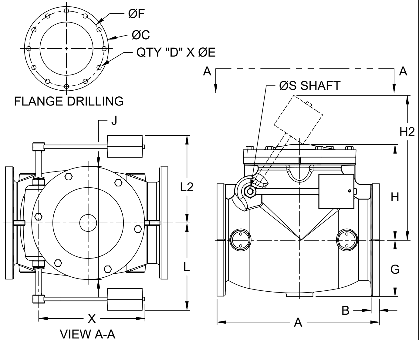
DIMENSIONS (Inches)
