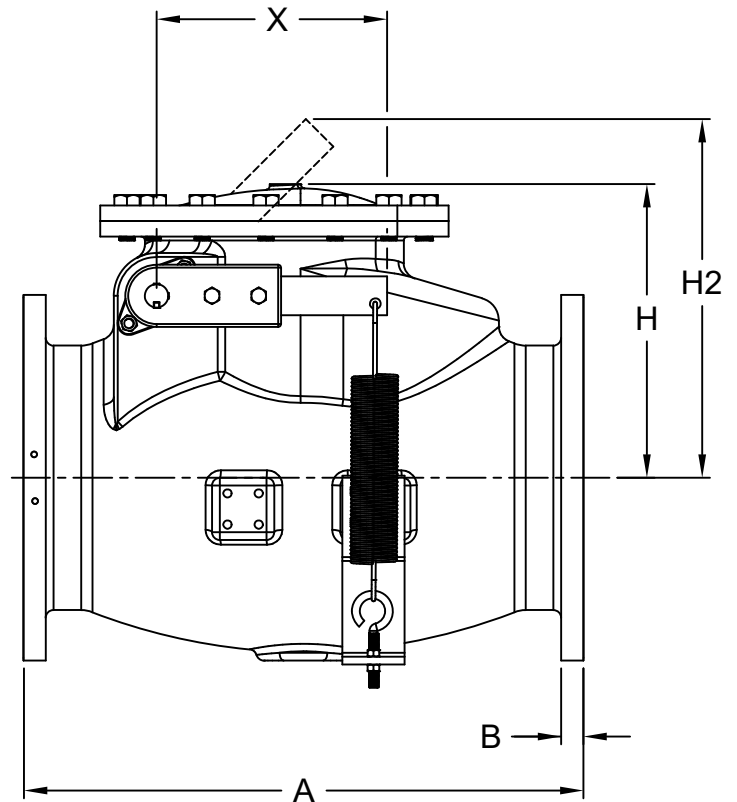
DIMENSIONS (Inches)
