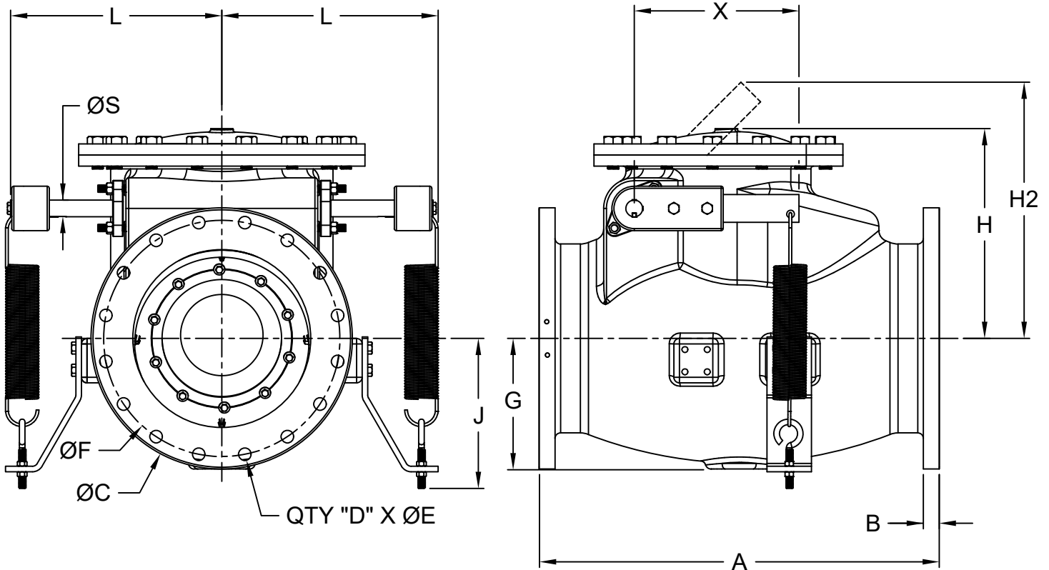
DIMENSIONS (Inches)
