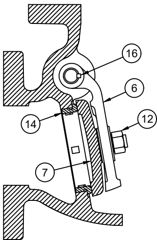
3" Metal Seated Check Valve
