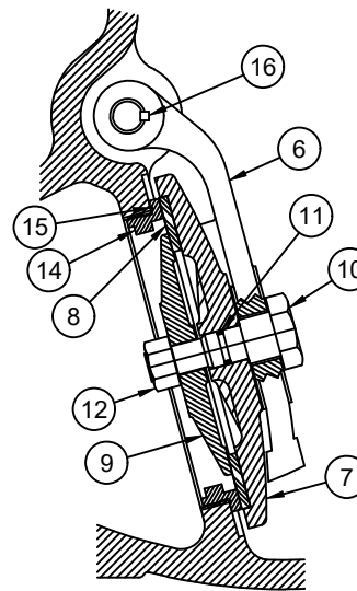
4"-12" Resilient Seated Check Valve
