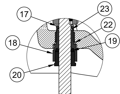
STUFFING BOX DETAIL
