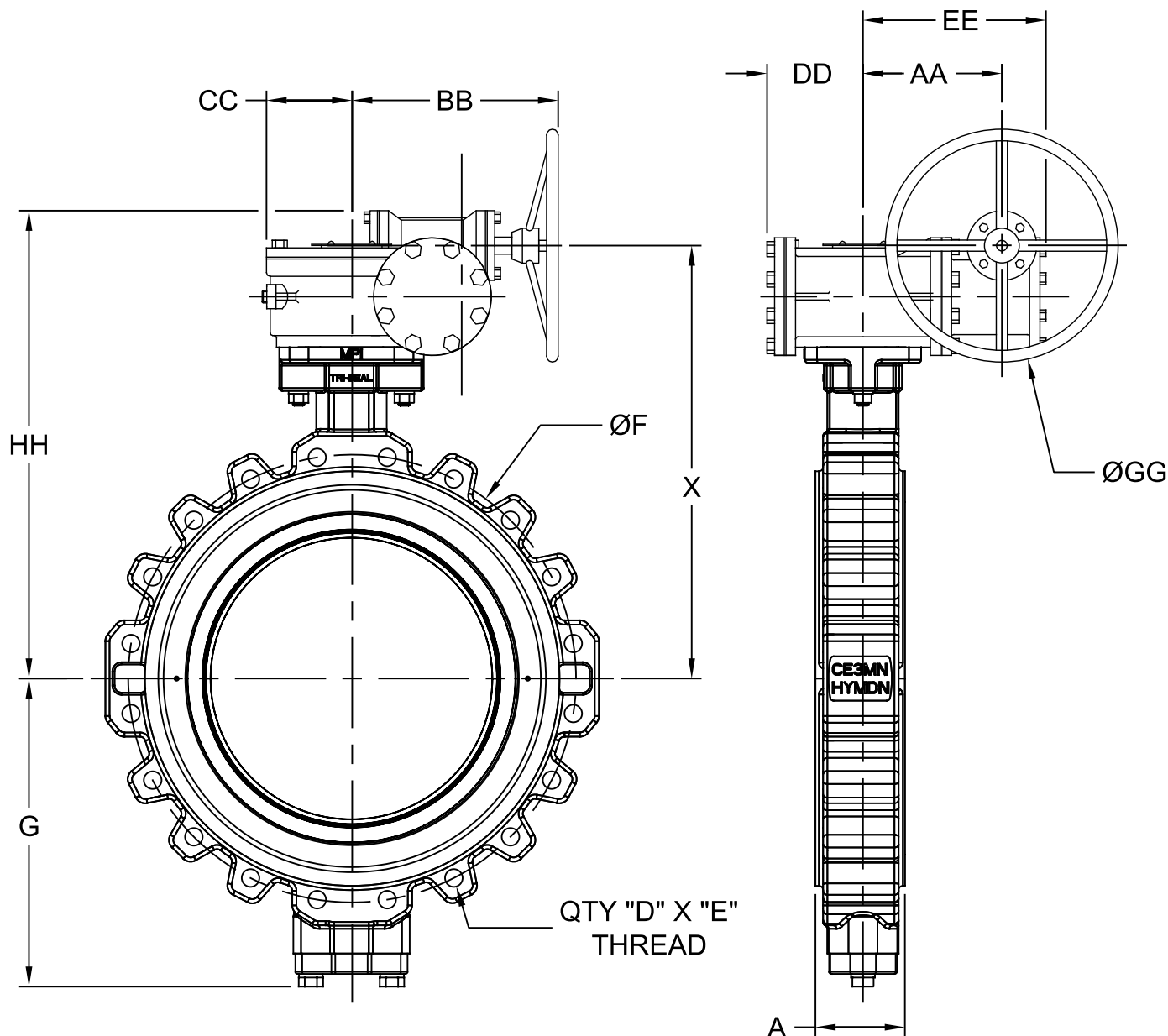
DIMENSIONS (Inches)
