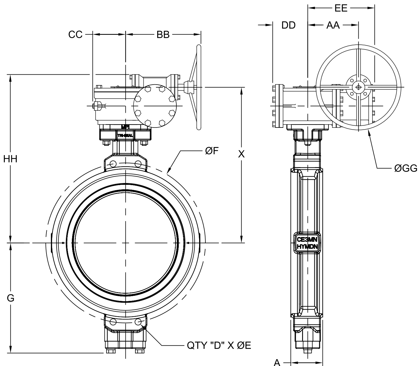
DIMENSIONS (Inches)
