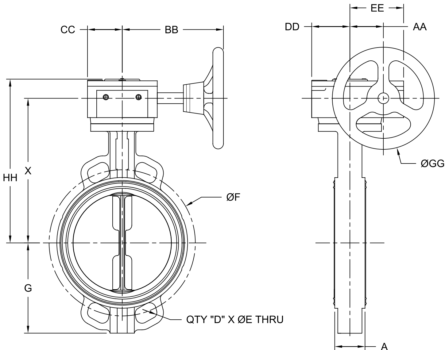
DIMENSIONS (Inches)
