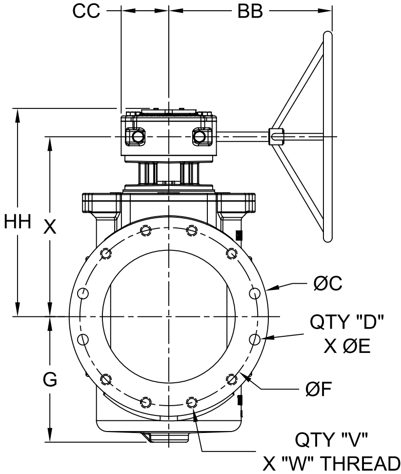
DIMENSIONS (Inches)
