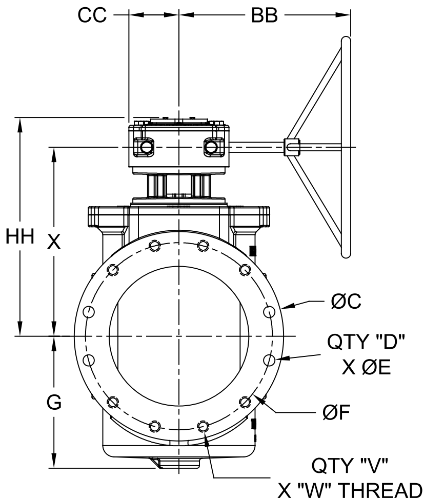
DIMENSIONS (Inches)
