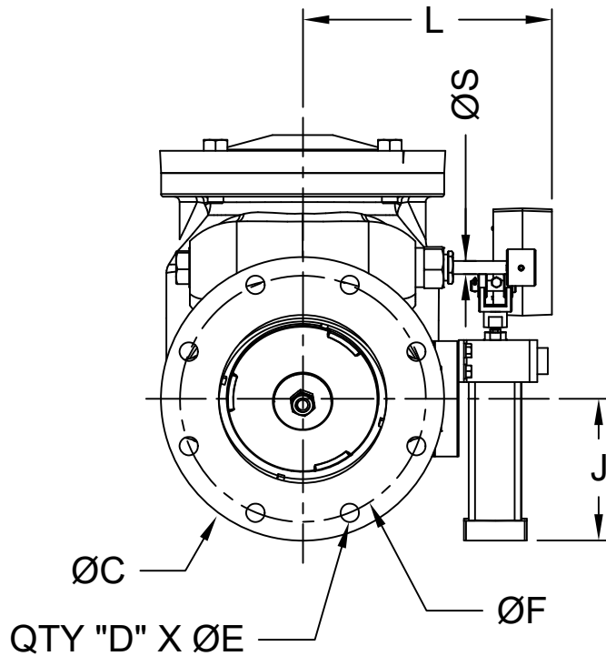
DIMENSIONS (Inches)
