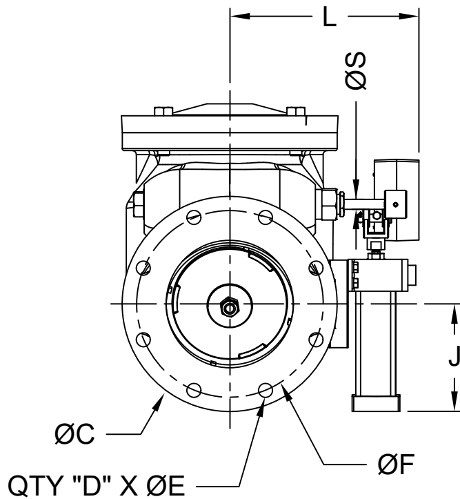
DIMENSIONS (Inches)
