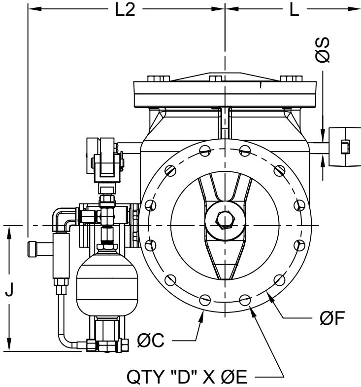
DIMENSIONS (Inches)
