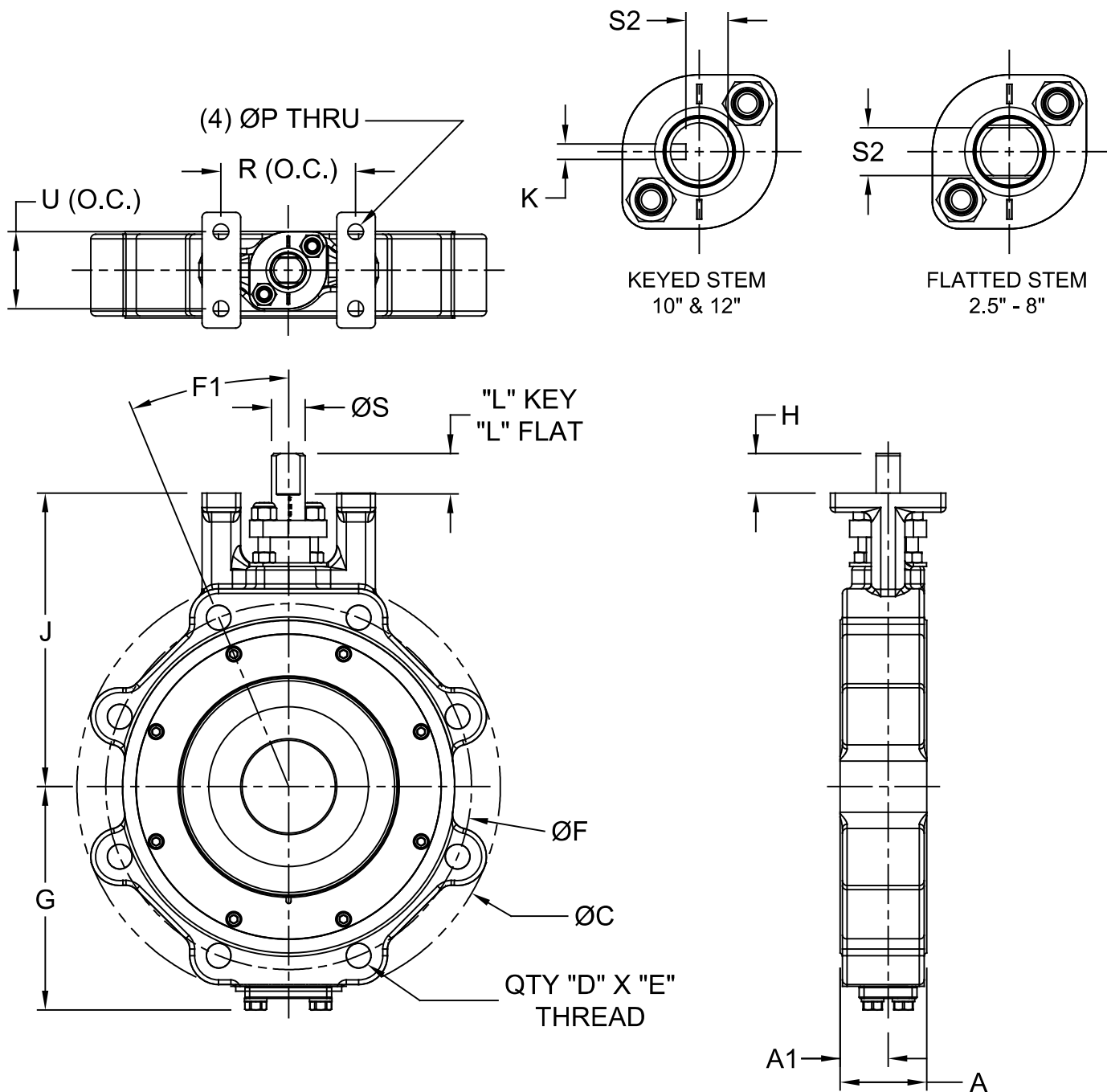
DIMENSIONS (Inches)
